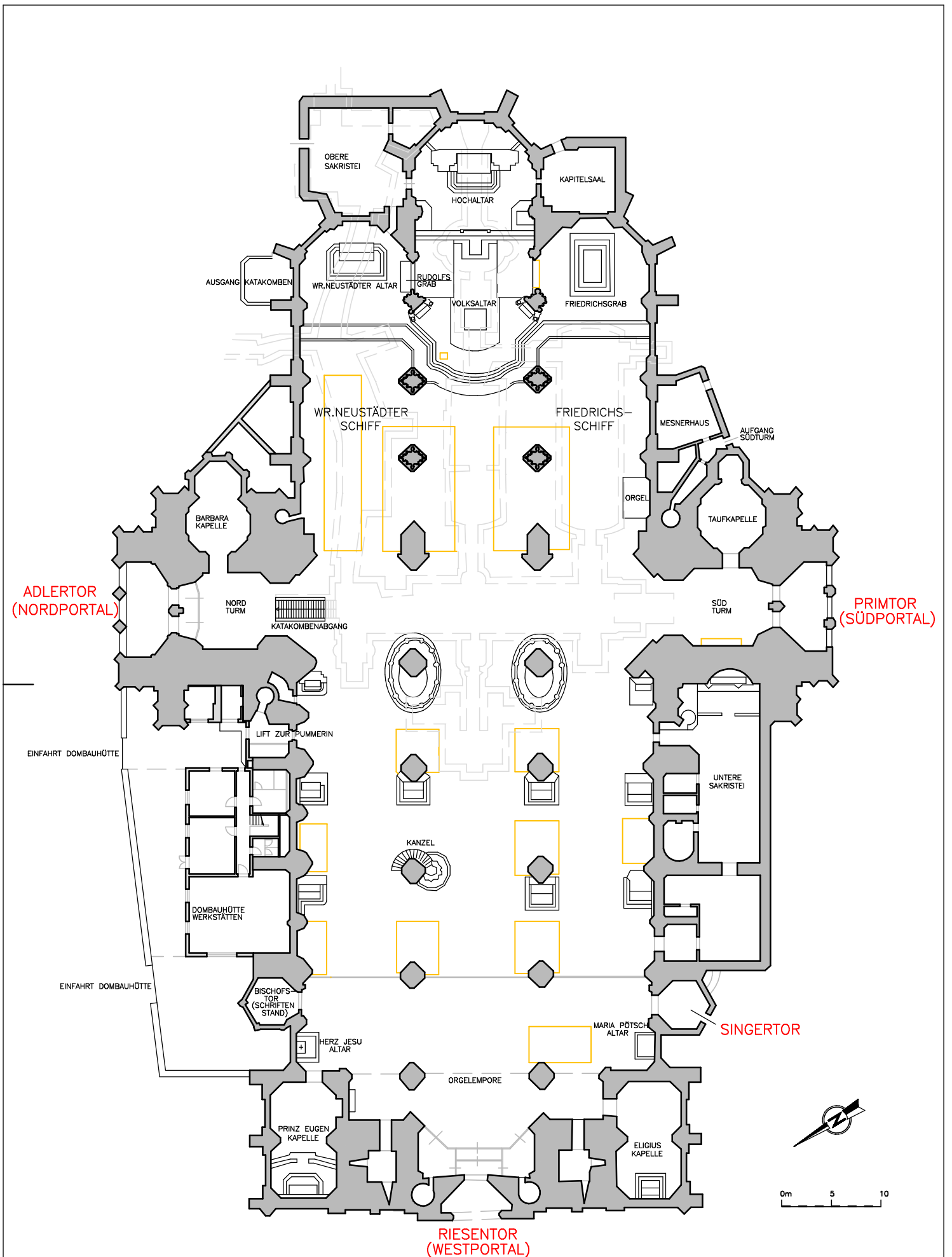
DOM ZU ST.STEPHAN, WIEN - GRUNDRISS ST.STEPHAN'S CATHEDRAL, VIENNA - FLOOR-PLAN
